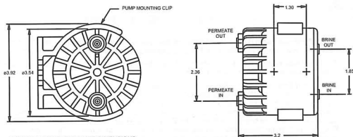
FIGURE 1. PERMEATE PUMP DIMENSIONS
